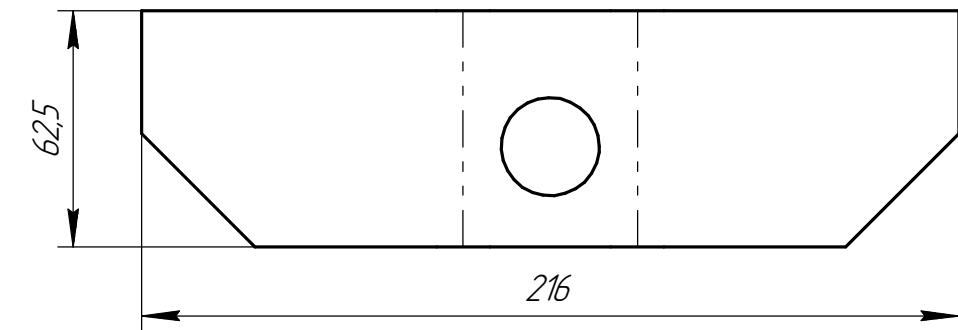
Q (1:2)
