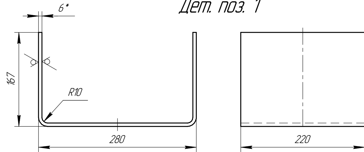
Q (1:5)
